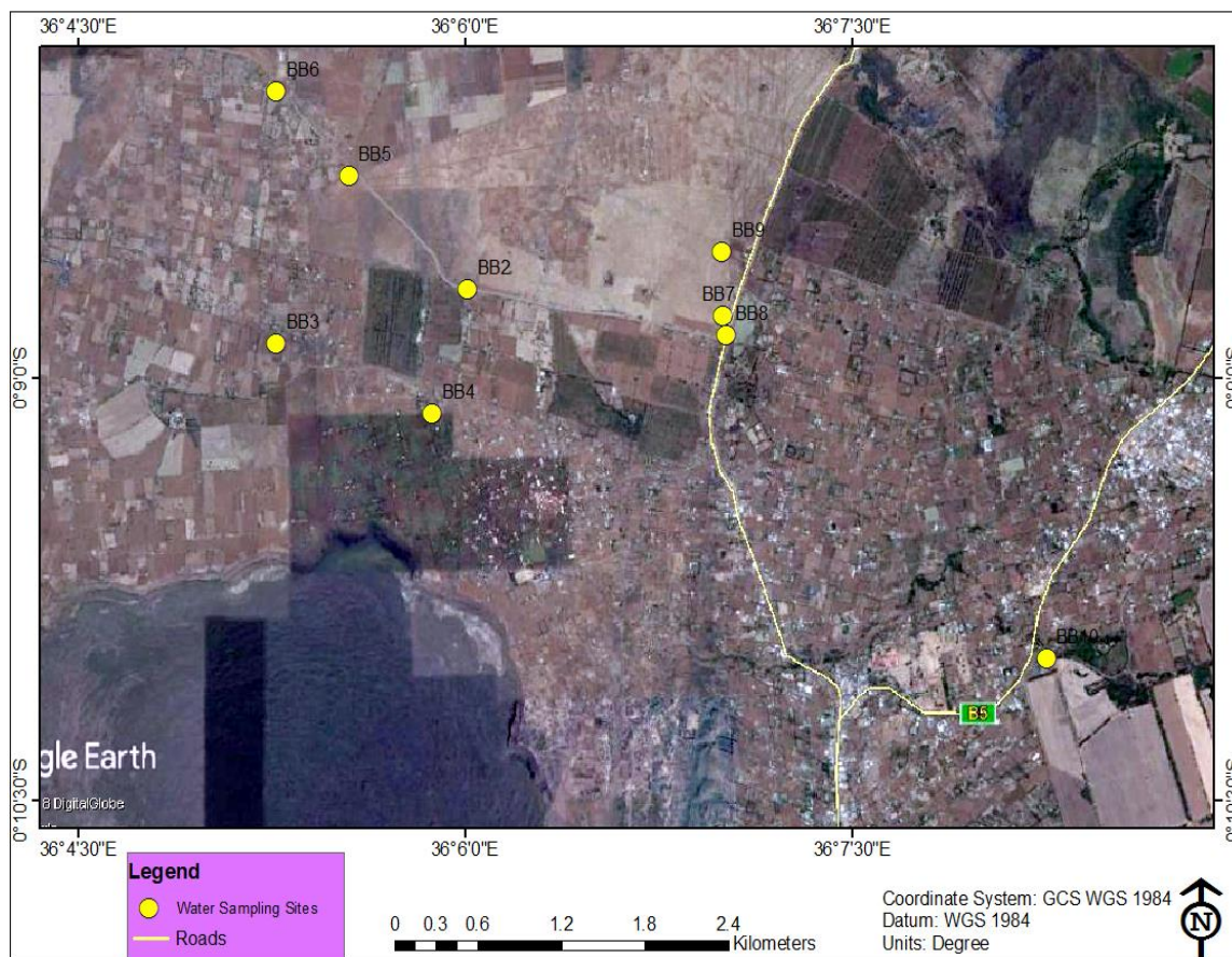
Figure 3: Location map of sampling points representing Olobanita well fields (BB2 to BB10) in Nakuru Municipality Source: Author's field work (2014 to 2015)
