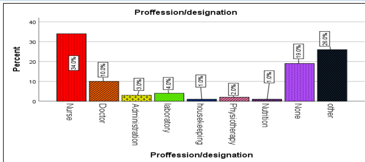
Figure 1: profession
