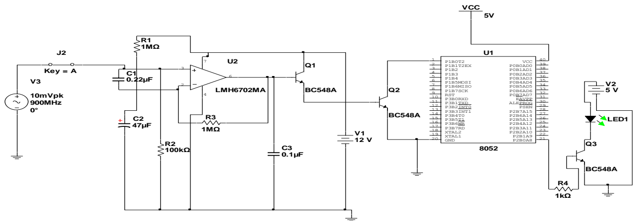
Figure 2: Detector circuit with buzzer and microcontroller
